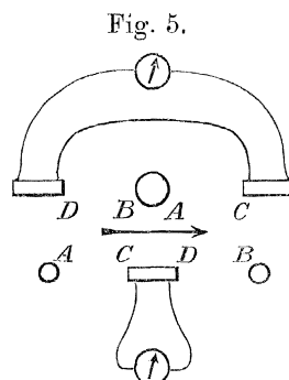
Fig. 5. Thermopile experiment suggested by FIZEAU; in two alternative forms.
